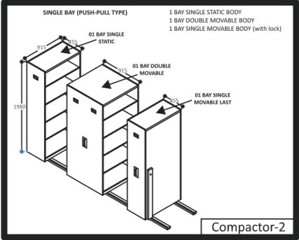
Push Pull Type Compactor COMPACTOR-2
